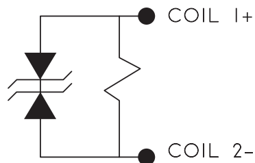
P/N 807/907 ZENER DIODE COIL SUPPRESSION -S-OPTION
