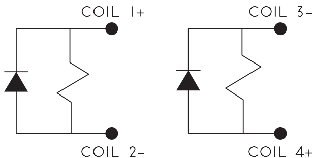
P/N 807/907 DIODE COIL SUPPRESSION W/ -F-OPTION
