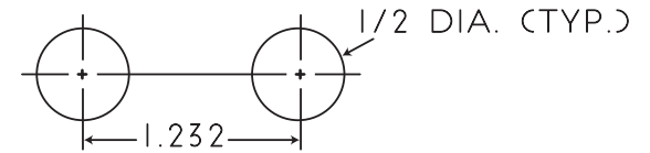
PANEL CUTOUT FOR TOGGLE SWITCH
