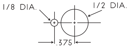
PANEL CUTOUT FOR TOGGLE SWITCH
